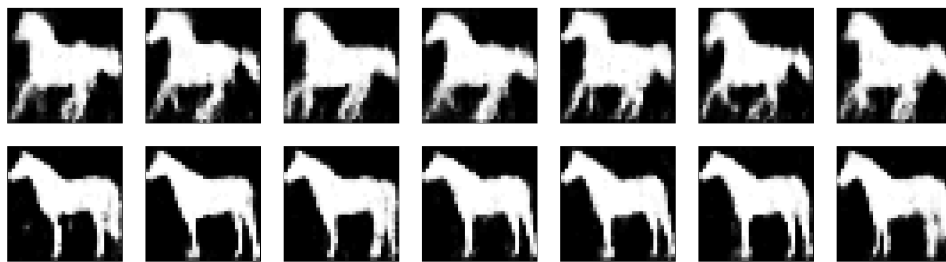
Figure 4.17: Clamped sampling. Sampling chains are run for two fixed, but different, configurations of h^2 . The horse’s pose remains fixed, but configurations of legs, and neck and back positions vary. This suggests that the highest layer in the model predominantly captures high-level pose information.
