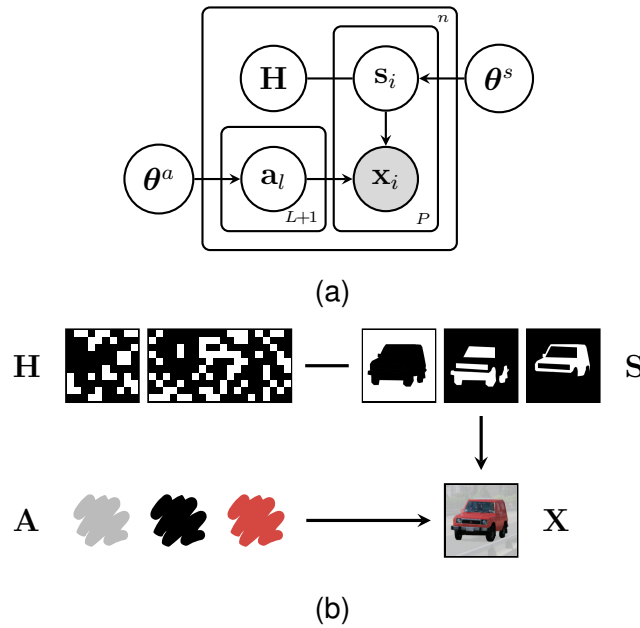
Figure 5.4: A model of shape and appearance. (a) The joint model. Pixels \mathbf{x}_i are modelled via appearance variables \mathbf{A}_l . The model’s belief about each layer’s shape is captured by shape variables \mathbf{H} . Segmentation variables s_i assign each pixel to a layer. (b) Schematic for an image \mathbf{X} .
