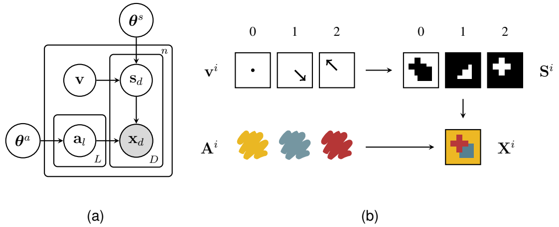
Figure 3.4: The Factored Shapes and Appearances model. (a) Directed graphical representation of the global FSA model. Pixel intensities x_i are modelled via L appearance random variables ( a_l ). The model’s belief about each part’s shape is captured by a latent variable ( v ). Here v represents the slight translation of the cross and square, but in theory it can represent any kind of deformation. Segmentation random variables ( s_i ) assign each image pixel to a part. (b) Schematic diagram of the model for a single image X^d .
