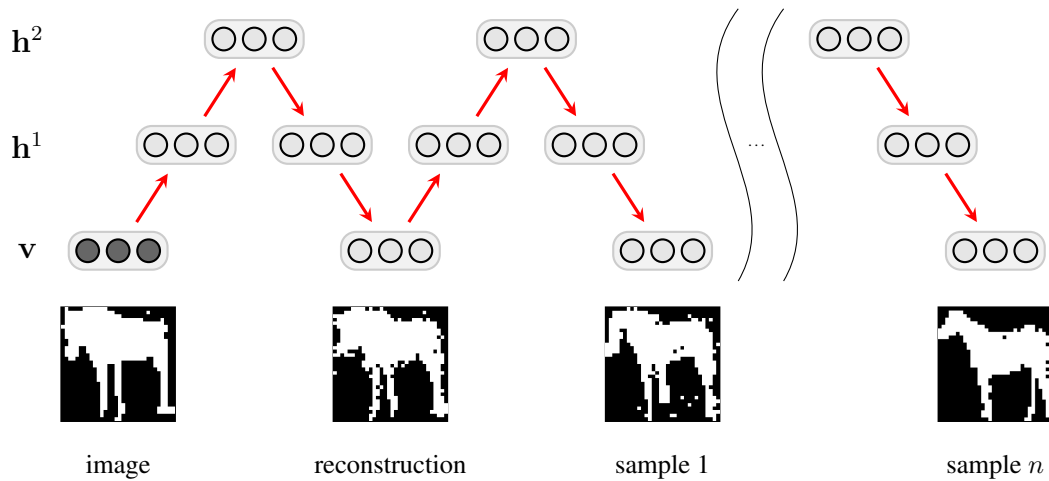
Figure 4.5: DBM Markov Chain Monte-Carlo . Block-Gibbs MCMC sampling scheme, in which v , h^1 and h^2 variables are sampled in turn. Note that each sample of h^1 is obtained conditioned on the current state of v and h^2 . For sufficiently large values of n , sample n will be uncorrelated with the original image.
