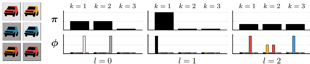
Figure 5.3: Appearance modelling using mixtures of histograms. Left: An exemplar dataset. Here we assume one background ( l = 0 ) and two foreground ( l = 1 , non-body; l = 2 , body) parts. Right: The corresponding appearance model. In this example, L = 2 , K = 3 and W = 6 . Best viewed in colour.
