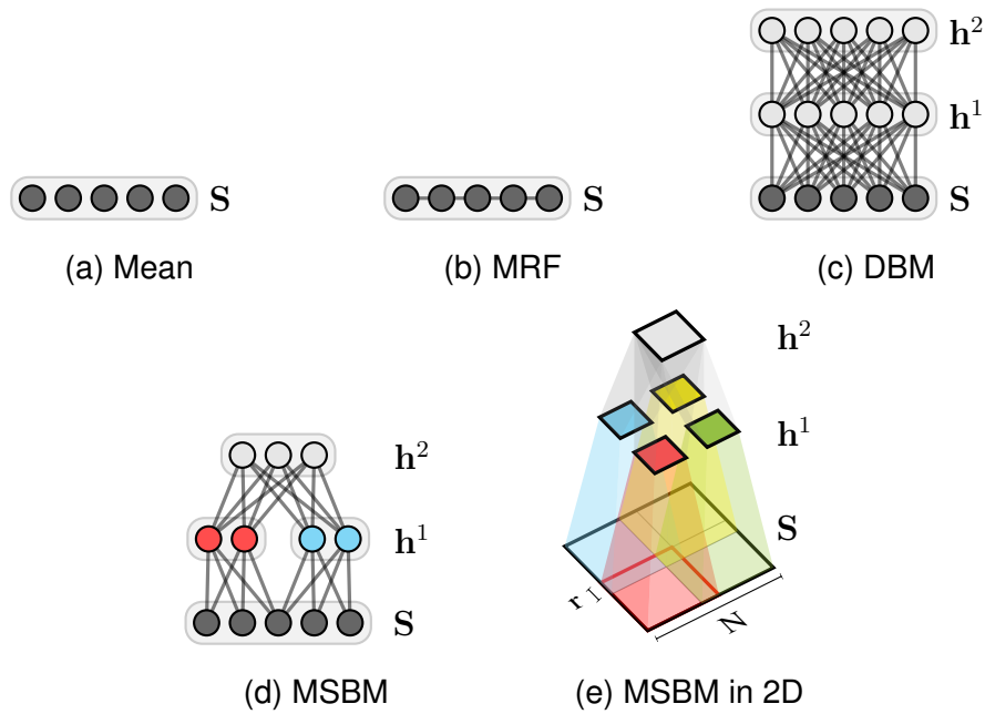
Figure 5.2: Models of shape. Object shape is modelled with undirected graphical models. (a) 1D slice of a mean model. (b) Markov random field in 1D. (c) Deep Boltzmann Machine in 1D. (d) 1D slice of a Shape Boltzmann Machine. (e) Shape Boltzmann Machine in 2D. In all models latent units h are binary and visible units S are multinomial random variables.
