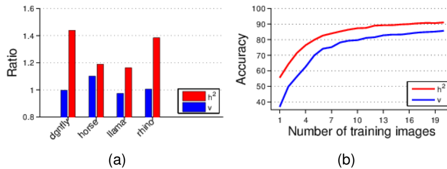
Figure 4.20: Classification using the learned representation. (a) The ratio of inter- and intra-class distances (values > 1 indicate that inter-class distances are larger). (b) GLM classification accuracy as a function of the number of training images, averaged over 100 runs.
