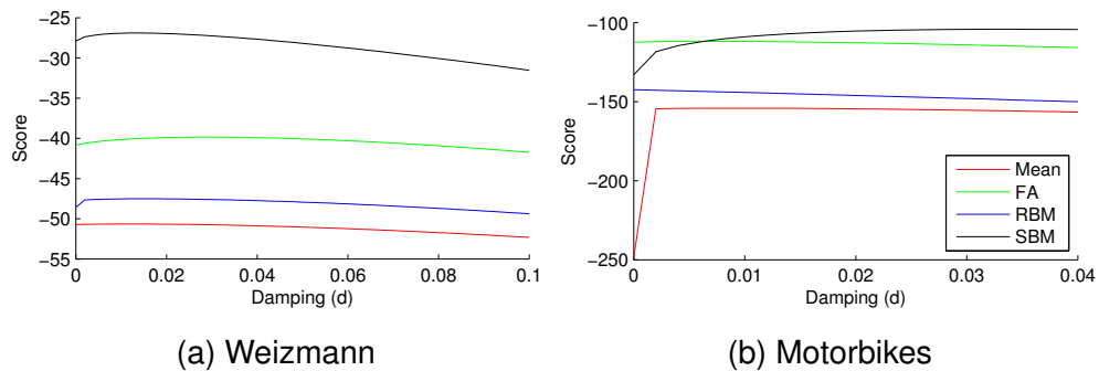
Figure 4.14: The effect of damping on imputation scores. The damping ranges have been chosen to ensure that the d at which the maximum score is achieved by each method is visible in the plots.
