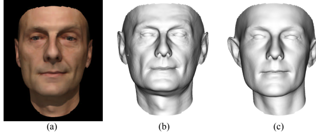
Figure 1.3: (a) Input rendered image, b) Ground truth and c) Shape estimated using a state-of-the-art model fitting algorithm [76]. The algorithm uses an analysis-by-synthesis technique to optimise an objective comprising three error terms based on landmark points, contours and image intensity. In spite of using this state-of-the-art model fitting approach, the estimated shape fails to capture all the atypical features of the face (wrinkles on the cheek). This clearly emphasises model dominance as a serious weakness and shows the need to study additional cues to overcome this drawback.
