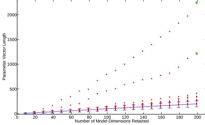
Figure 4.3: Parameter vector length vs Number of model dimensions retained. The red points represent the vector length for each out-of-sample face. The error bars (blue) represent three standard deviation variation around the mean of the chi-square distribution. The green squares denote the two faces which grossly overfit when projected onto the model (see column (b) in Figure 4.6).
