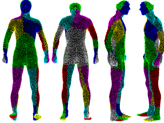
Figure 2.5: A body mesh partitioned into 30 charts. The various colours represent the vertices belonging to the respective charts.
