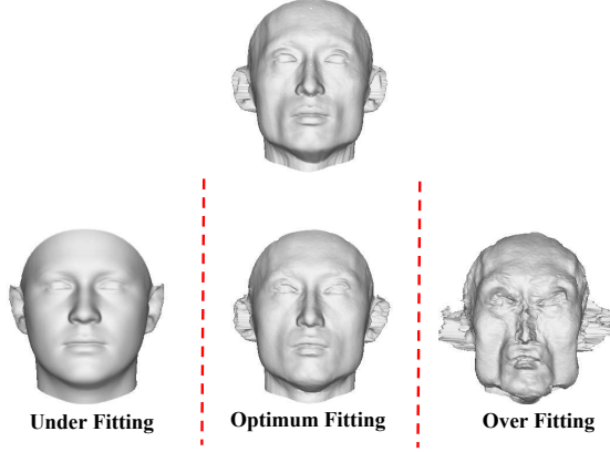
Figure 3.7: Shows the tradeoff between the fitting quality and shape plausibility. Given an unseen face (top row), the bottom row shows the three cases of fitting: (a) Under Fitting (b) Optimum Fitting and (c) Over Fitting.
