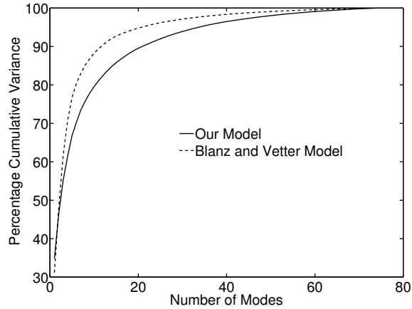
Figure 3.3: Cumulative variance curve.
