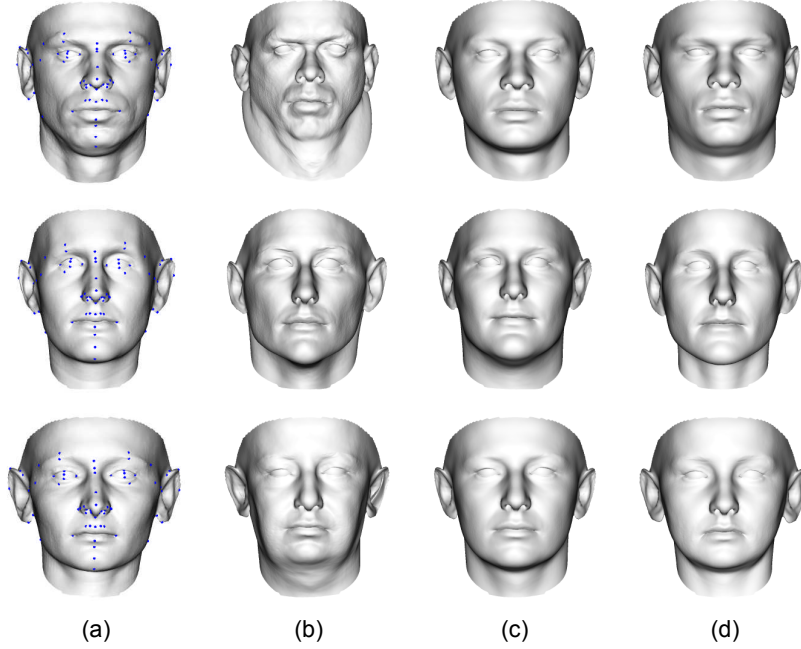
Figure 4.12: Underconstrained model fitting example: (a) ground truth faces (unseen) with the input feature points (blue circles); (b) LMA with no regularisation constraint; (c) LMA with regularisation constraint; (d) manifold optimisation. All the results are for a n = 50 parameter model.
