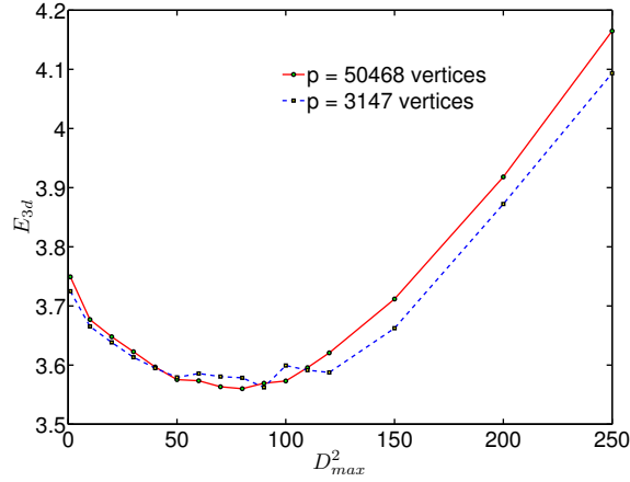
Figure 3.8: E_{3d} (in mm) vs D_{max}^2 .
