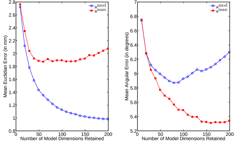
Figure 4.5: Left plot (a): Mean Euclidian error vs Number of model dimensions retained; Right plot (b): Mean angular error vs Number of model dimensions retained. All reported error measures are averaged over the 10 unseen faces in the BFM.
