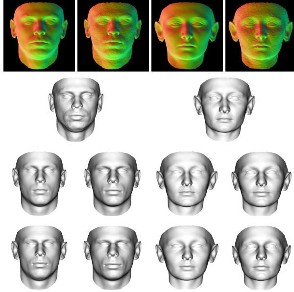
Figure 5.5: Model fitting estimates (optimising Equation 5.18). Row 1 shows the input bump maps (noise free and noisy) for 2 unseen subjects. Row 2 shows the ground truth. Row 3 shows the shape estimates obtained using the model at the highest resolution. Row 4 shows the shape estimates obtained using the model at a resolution of 5000.
