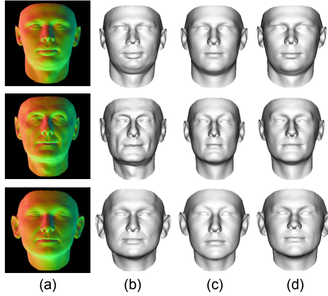
Figure 4.11: Overconstrained model fitting example: (a) input bump maps for 3 unseen subjects; (b) ground truth; (c) BFGS optimisation; (d) manifold optimisation. All the results are for a n = 99 parameter model.
