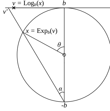
Figure 4.2: Computing log and exponential maps using a stereographic projection for the S^1 manifold.
