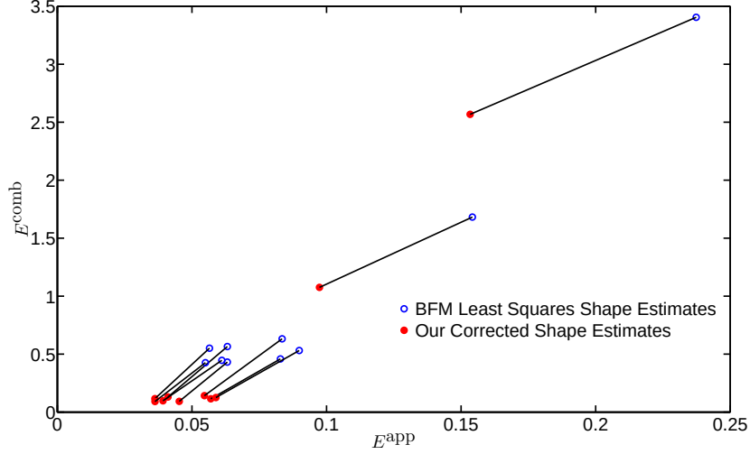
Figure 6.1: E^{\text{comb}} (in \text{mm}^2 ) vs E^{\text{app}} (in normalised squared pixel intensity).
