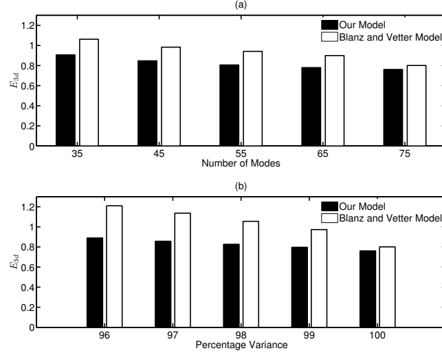
Figure 3.5: (a) E_{3d} (in mm) vs Number of modes, (b) E_{3d} (in mm) vs Percentage variance.
