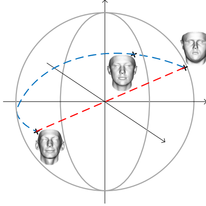
Figure 4.7: Warping between face and antiface on the S^2 manifold. A linear warp is shown in red and one of the possible plausibility-preserving warps is shown in blue.
