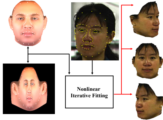
Figure 3.6: Framework for the proposed system. The mean mesh (top left) and 2D input image with k indexed annotations (center) are the inputs to the system. The mean texture map (bottom left) is used to determine the vertices (white dots) corresponding to the k indexed points (yellow dots) in the input image. The system outputs the estimated shape and pose (right column). A simple blending function is used to estimate the occluded texture. The 2D input image is taken from [93].
