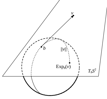
Figure 4.1: Exponential map for the S^2 manifold.
