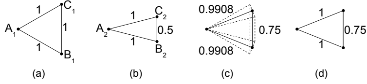
Figure 2.3: Averaging optimal parameterisations does not yield optimal results. (a) and (b) show two triangles flattened with zero distortion. (c) shows the Euclidian average of the two flattenings with \sigma_1 = 0.1575 . (d) shows the optimal result with \sigma_1 = 0.1562 .
