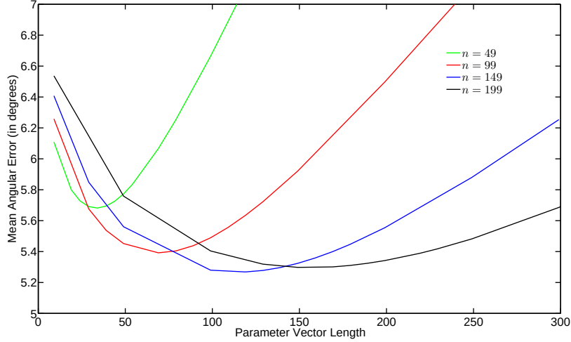
Figure 4.4: Mean angular error vs Parameter vector length (for four different values of model dimensions retained). All reported error measures are averaged over the 10 unseen faces in the BFM.
