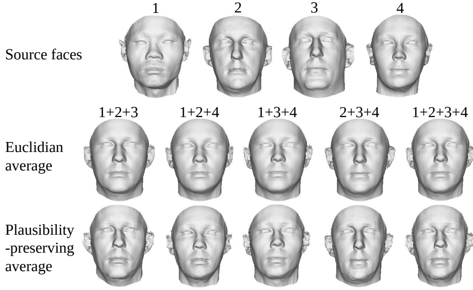
Figure 4.10: Linear versus plausibility-preserving averages.
