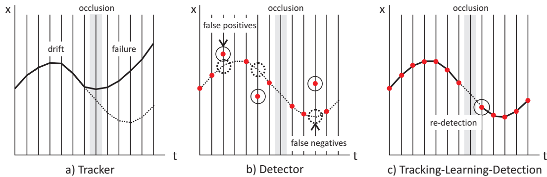
Figure 6.1: Illustration of a tracker (a), detector (b), and a tractor (c). Dotted line shows ground truth trajectory, gray bar represents full occlusion, thick line is the trajectory of a tracker, red dots are responses of a detector.
