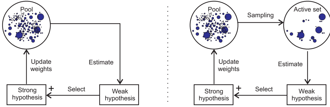
Figure 4.1: Illustration of standard boosting (LEFT) and boosting combined with bootstrapping (RIGHT).
