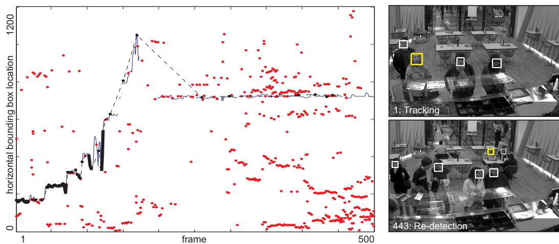
Figure 6.11: Evaluation of Face-TLD on sequence Surveillance. (LEFT) Responses of generic face detector (red), detections approved by online learned model (black), ground truth trajectory of the subject (blue). (RIGHT) The surveillance scenario.
