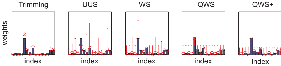
Figure 4.3: Pool with weights d_i (blue bars) is repeatedly sampled to obtain a distribution of the estimated weights. The range of the distribution (1 and 99% quantiles) is depicted by red vertical lines and expected values by circles.
