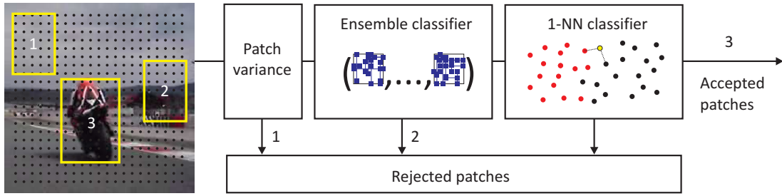
Figure 6.4: The block diagram of the object detector.
