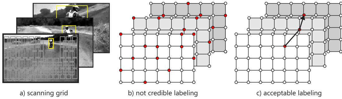
Figure 5.7: Illustration of a scanning grid applied to three consecutive frames (a) and corresponding spatio-temporal volume of labels with unacceptable (b) and acceptable (c) labeling. Red dots correspond to positive labels.
