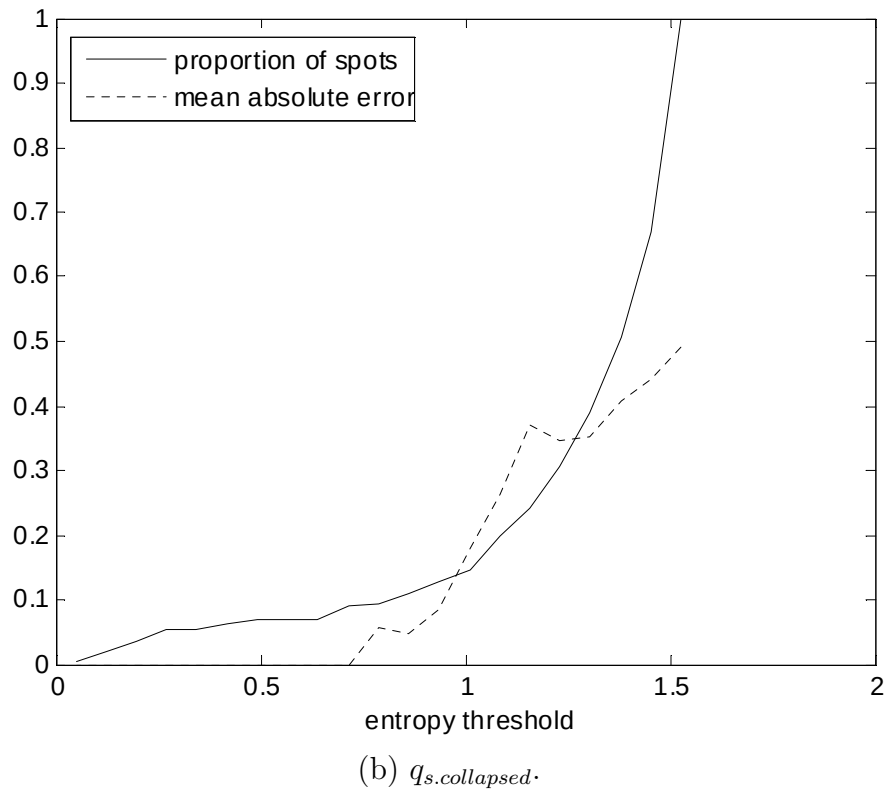
Figure 6.7: Fraction of scored spots and associated mean absolute error, for different entropy thresholds and for both quickscore values. From the experiments based on expectation propagation and Gaussian kernels. (Lower entropy means higher confidence.)
