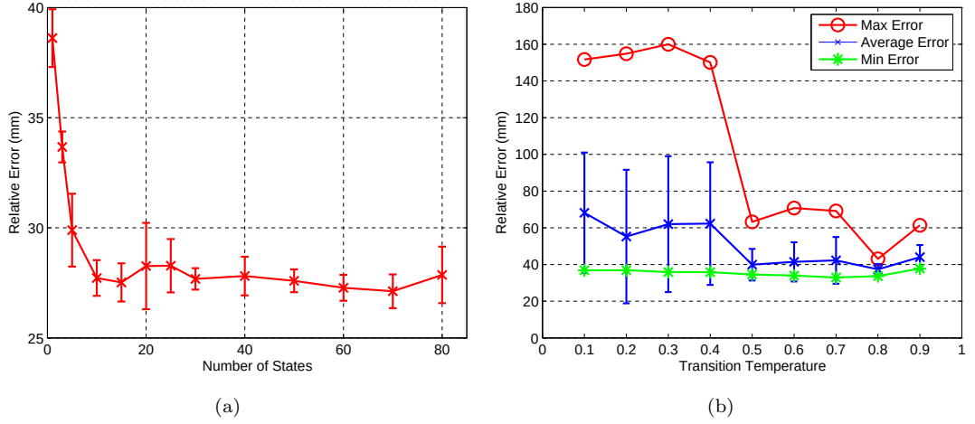
FIGURE 4.9: Range data simulation results: (a) mean tracking error versus number of states; (b) tracking error versus transition temperature \rho_T .
