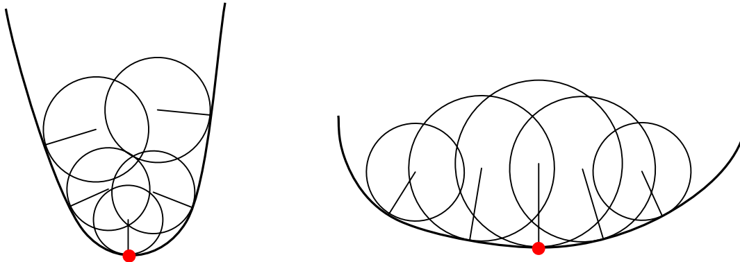
Figure 51: Vertices on a curve. Left: Maximal vertex (radius of circle of curvature becomes minimum, therefore curvature becomes maximum). Right: Minimal vertex (radius of circle of curvature becomes maximum, therefore curvature becomes minimum). The equivalent in 3D are the ridges as defined in this section.
