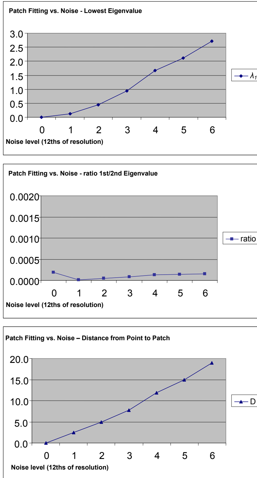
Figure 25: Graphs for the mean values of the evaluation metrics for the test ellipsoid with increasing levels of noise.
