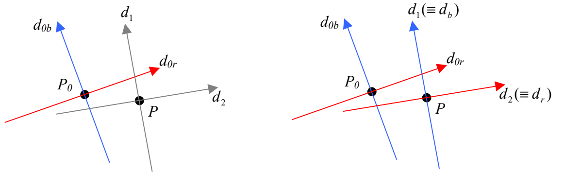
Figure 29: Propagation of red and blue curvature labels based on the directions of principal curvature. Left: Before. Right: After.
