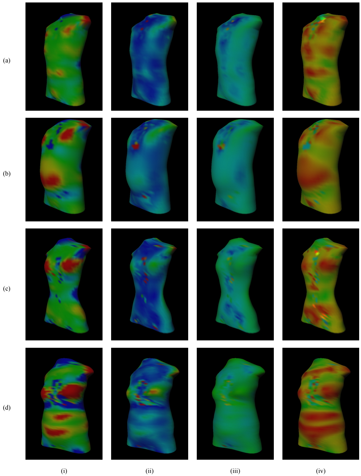
Figure 35: Results for scans of human torsos (front view). By row: Thin male, fat male, thin female, fat female. By column: Gaussian curvature, mean curvature, curvedness, shape index.
