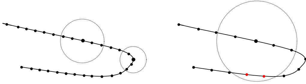
Figure 6: Sufficient vs. Insufficient Sampling. Left: The shape is sufficiently sampled. A circle centered on a sample and large enough to contain the sample's immediate neighbours contains no other samples. Right: The shape is insufficiently sampled. A circle centered on a sample and large enough to contain the sample's immediate neighbours contains also points that do not belong to the neighbourhood (shown in red). These can be filtered out if the ordering of the samples is known (i.e. if they arose from the sampling of a parametric curve or surface). This is impossible if the ordering is unknown (i.e. if they are obtained by scanning a real object).
