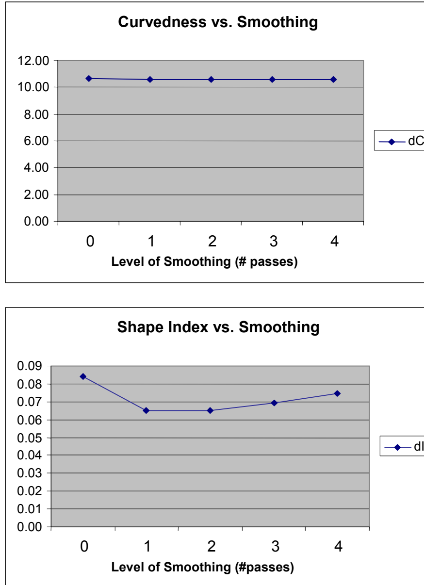
Figure 47: Graphs for the mean values of the absolute differences between calculated and actual values of the curvedness and shape index for a noisy ellipsoid with increasing levels of smoothing.
