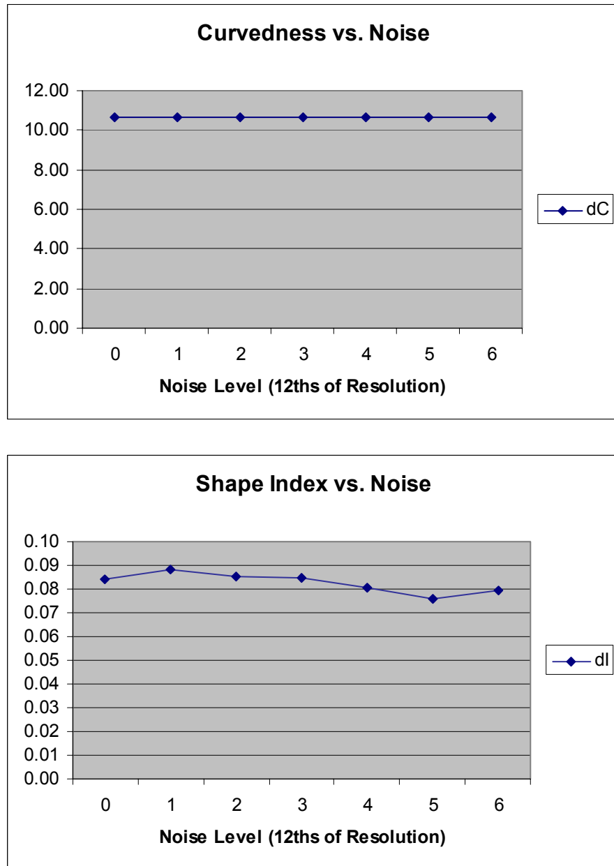
Figure 45: Graphs for the mean values of the absolute differences between calculated and actual values of the curvedness and shape index for the test ellipsoid with increasing levels of noise.
