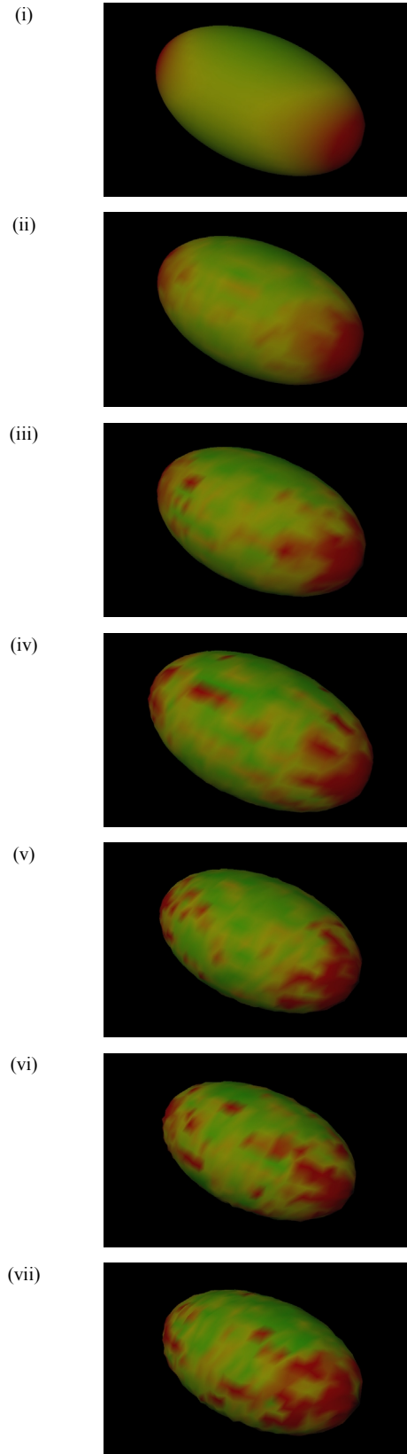
Figure 43: Behaviour of the curvature calculation algorithm on an ellipsoid with varying levels of uniform noise with amplitude ranging (top-to-bottom) from no noise at all to a level of 50% of the sampling resolution, at equal increments of 1/12^{\text{th}} of the resolution.
