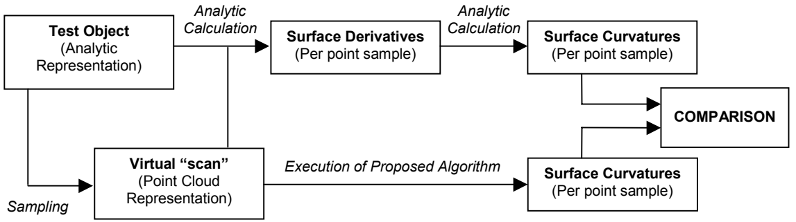
Figure 11: Diagram of the overall evaluation strategy.
