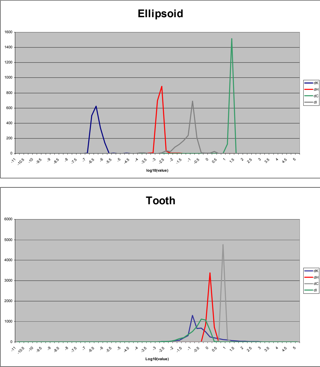
Figure 42 (part 1 of 2):Histograms of differences between the actual values of curvature properties on the test objects, and the values obtained via the fitted quadric patches.
