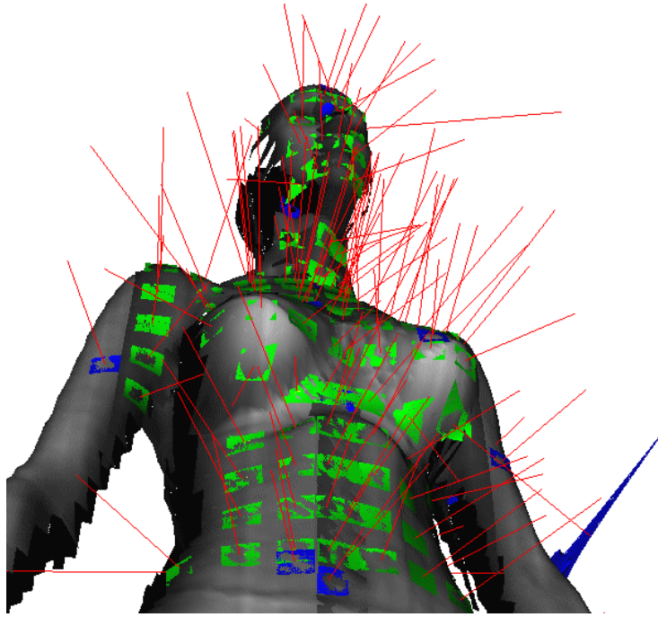
Figure 3: Fitting conic sections to body scanner data using the 3D extension of the method described in [Book79] (green: quadratic patch, blue: cubic patch – red lines illustrate the local surface normals calculated from the patches.). The poor quality of the result is evident when the data set corresponds to a synclastic (elliptic) shape.
