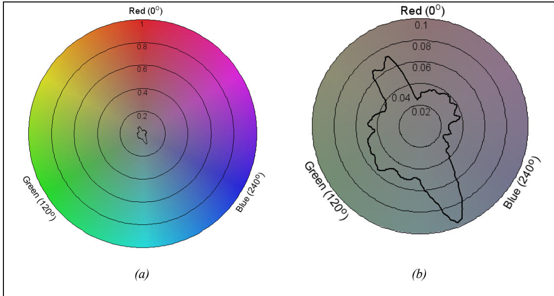
Figure A-13 – (a) A horizontal slice of the HLS colour space at L = 128 . The centre area marks the colours considered achromatic based on the measurements made. A magnification of the centre area is shown in (b). The slices appear cyclical instead of hexagonal here for illustrative purposes.
