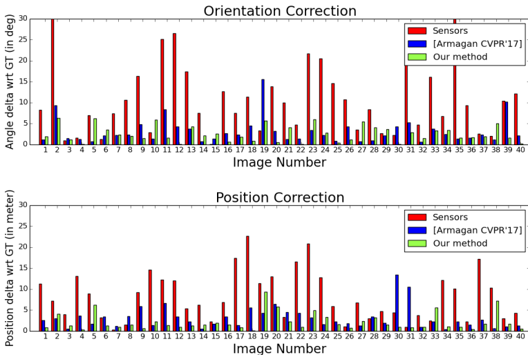
Figure 4: Orientation and location errors for the poses from the sensors, the poses obtained by [10], and the poses obtained by our method.
