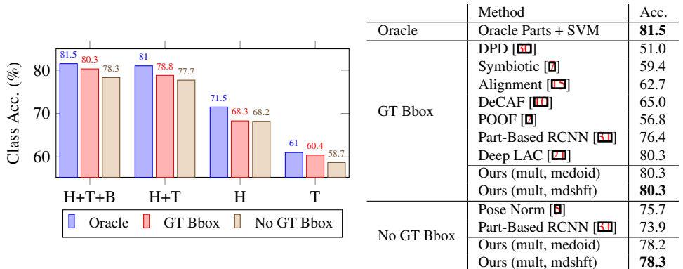
Figure 4: On the left we show a comparison of classification accuracies obtained using combinations of parts localized under different conditions (H: Head, T: Torso, B: Whole Body). On the right, we compare our classification accuracy with other works.
