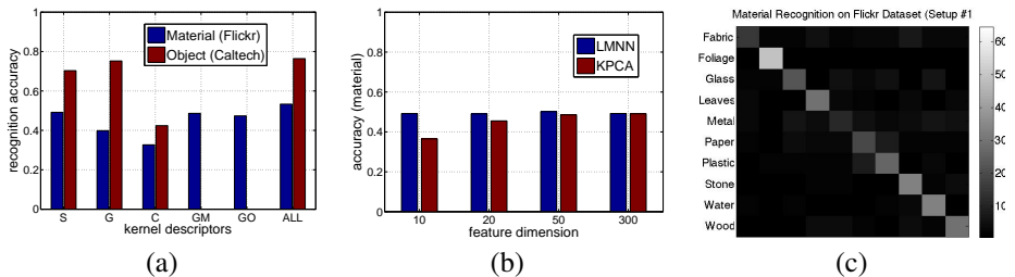
Figure 2: Results on MIT/Flickr. (a) Material recognition accuracies of five kernel descriptors with LMNN=10; with object recognition accuracies on Caltech 101 from [16]. (b) Accuracy vs dimension in LMNN for the best performing descriptor (shape), compared to kPCA. (c) Confusion matrix for material recognition using combined features.
