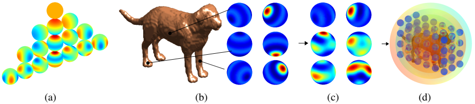
Figure 1: The basic ideas: (a) Spherical harmonics for representing HOG (real part of the first 4 bands are shown). (b) Individual gradient as function on a sphere (reconstructed from the SH coefficients). (c) The spatially aggregated spherical HOG . (d) Spherical tensor operations create rotation-invariant descriptions from the spherical HOG field .
