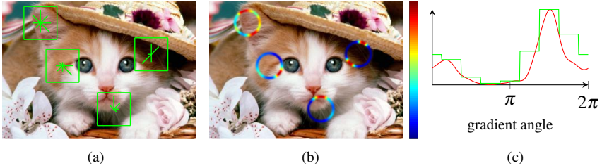
Figure 2: (a) Histogram of oriented gradient (b) Circles representing the histograms (c) 1D illustration of the histogram at bottom (All the continuous signals are reconstructed from first 8 Fourier coefficients after Gaussian filtering in the frequency domain.)
