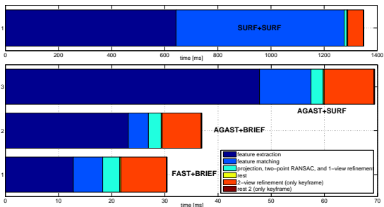
Figure 10: Timings of the different combinations of feature detectors and descriptors.
