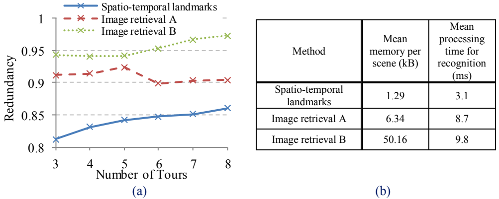
Figure 3: Comparison of (a) the database redundancy and (b) the computational requirements of recognition for our technique with that of the traditional image-retrieval approach, for the outdoor database, after 8 tours. The processing time excludes feature extraction and visual word assignment, which is consistent across all techniques.
