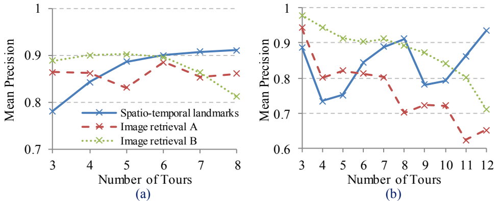
Figure 2: Comparison of the recognition precision of our technique with that of the image retrieval method in (a) outdoor scenes and (b) indoor scenes. Structural changes are manually made to the indoor scenes after 3 images are acquired, and again after 8.
