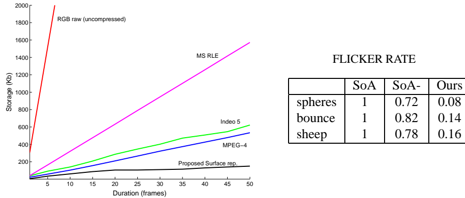
Figure 2: Left: Demonstrating the comparatively low storage requirements of the surface representation for up to 50 frames of a typical gradient-shaded cartoon animation. Right: Quantifying the lower rate of stroke flicker obtained via our method.
