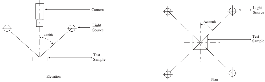
Figure 2: Image capture setup.
