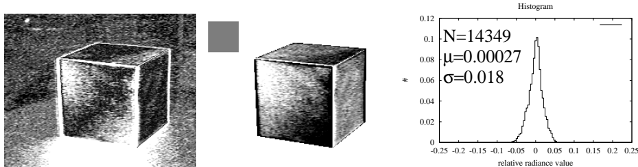
Figure 2: Comparison of original and synthetic images: The first image shows the absolute value of radiance differences multiplied by a factor of 30. In the ideal case the cube should be black. The second image shows the radiance differences multiplied by a factor of 20 and offset by the radiance value corresponding to the displayed square. In the ideal case the cube should have the intensity of the square. The histogram shows the distribution of the differences. The x-axis corresponds to the radiance difference and is normalised such that a value of 1 corresponds to the maximum radiance observed.
