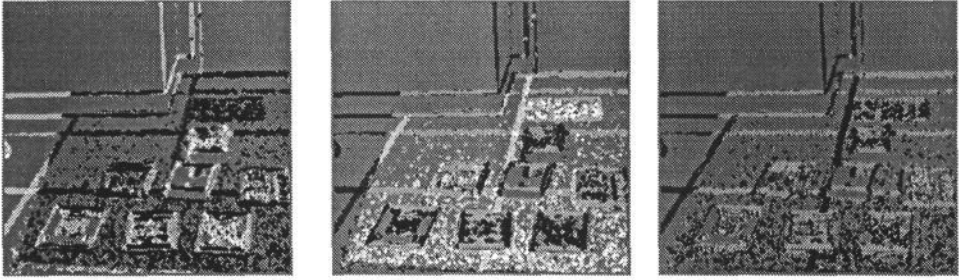
Figure 2: Log likelihood ownership maps for outliers (left), the floor model (middle), and for objects near the floor (right), consistent with the epipolar geometry (right), for the stereo pair in Figure 1. Here white corresponds to high likelihood, and the uniform grey background represents equal likelihood.
