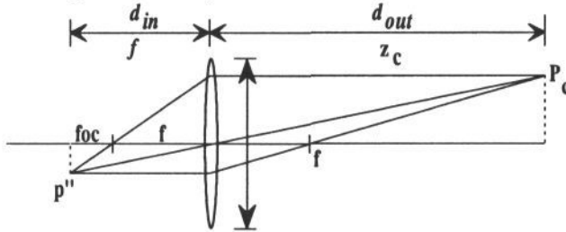
Fig. 3 - The Gauss lens model
