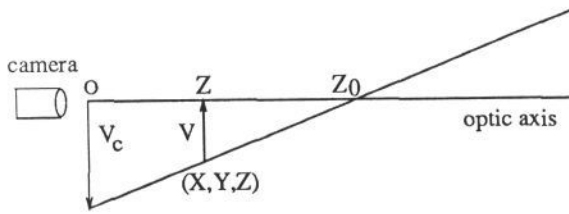
Figure 2: Geometry of kinetic depth
